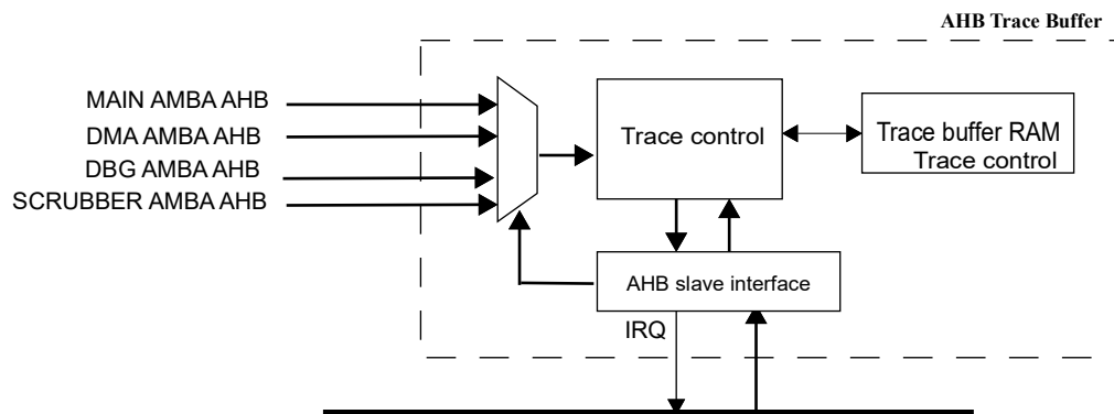
Figure 115. Block diagram
