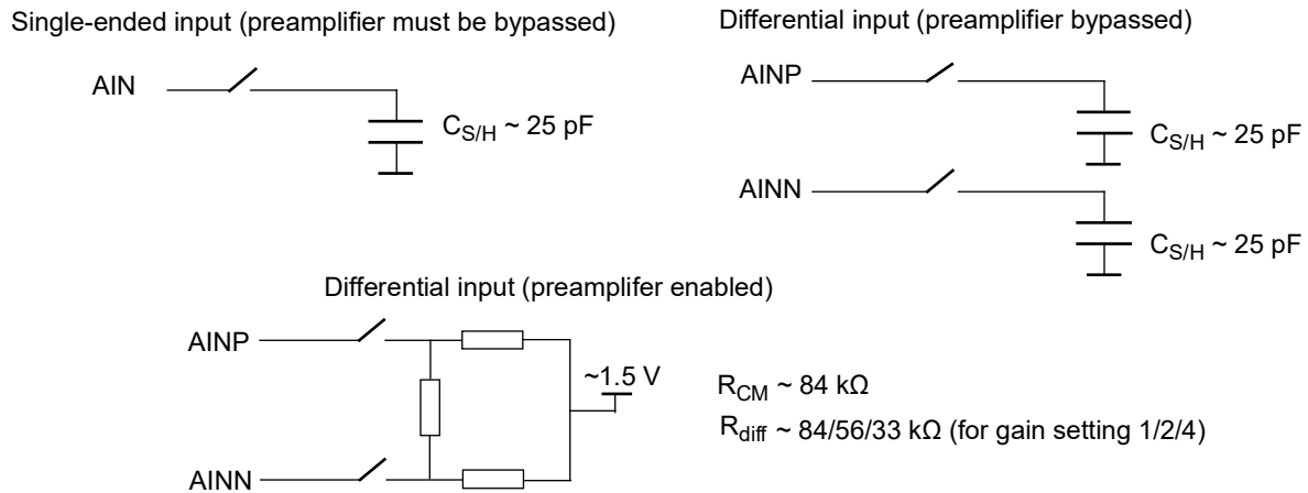
Figure 22. Simplified circuits of an ADC channel, with preamplifier bypassed or enabled.
