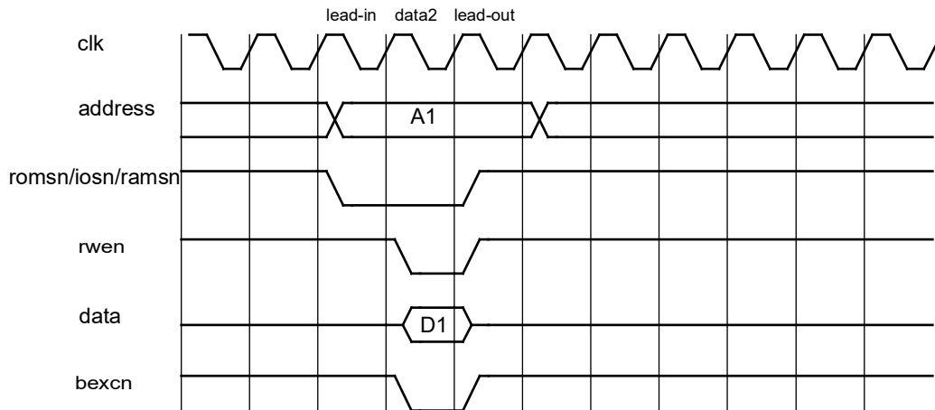
Figure 52. Write cycle with BEXCN. Chip-select (iosn) is not asserted in lead-in cycle for io-accesses.
