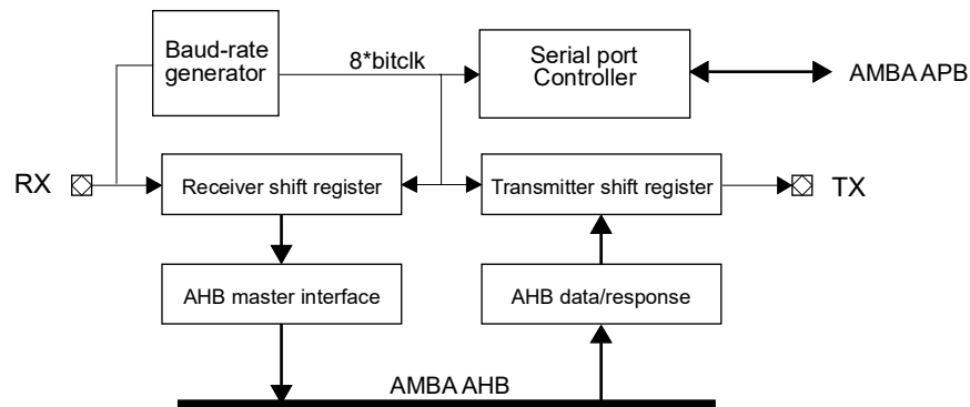
Figure 110. Block diagram
