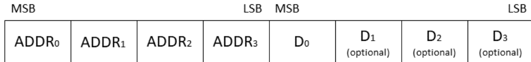
Figure 67. Use of data bytes in write commands (RPDO1 and RPDO3)
