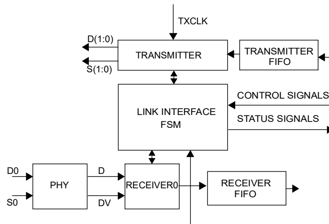
Figure 75. Block diagram
