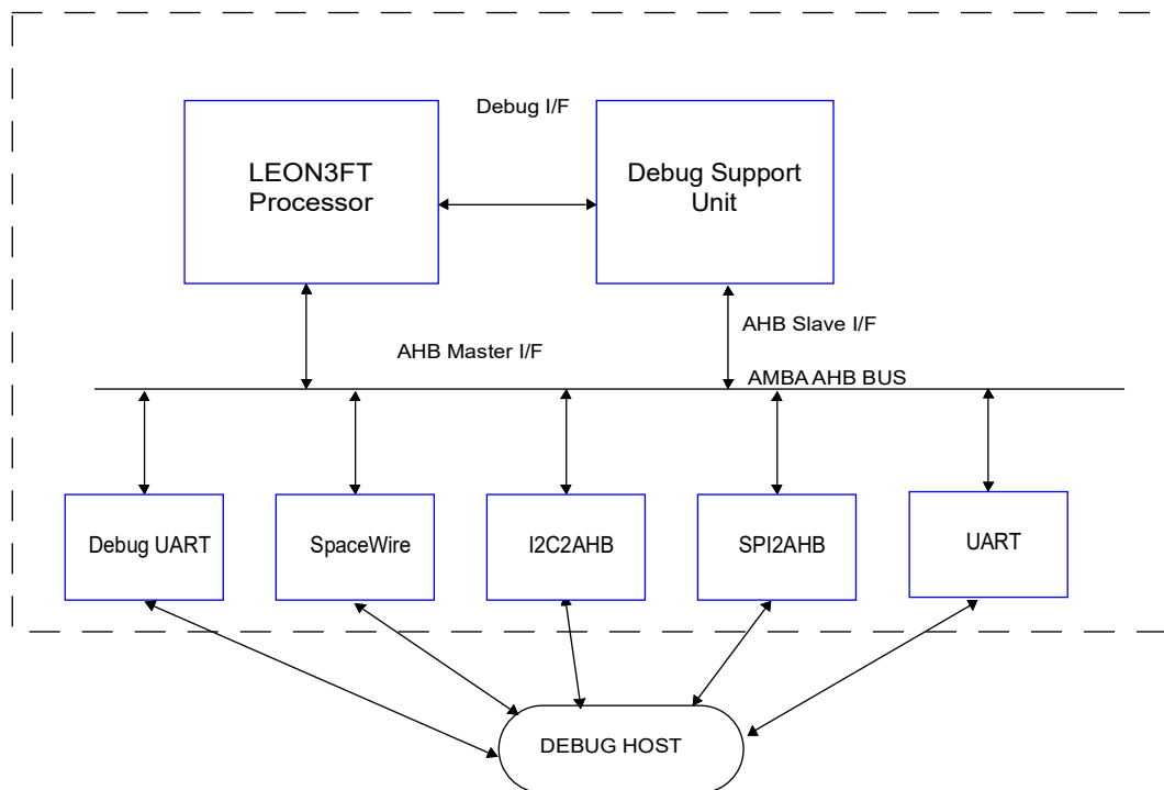
Figure 38. LEON3FT/DSU Connection
