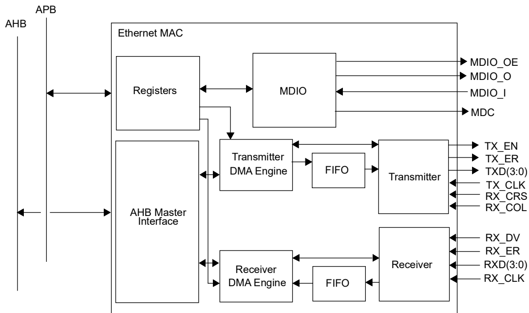
Figure 64. Block diagram of the internal structure of the GRETH.
