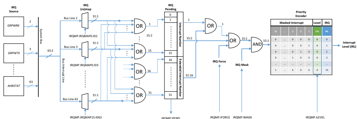
Figure 92. System and Interrupt controller block diagram
