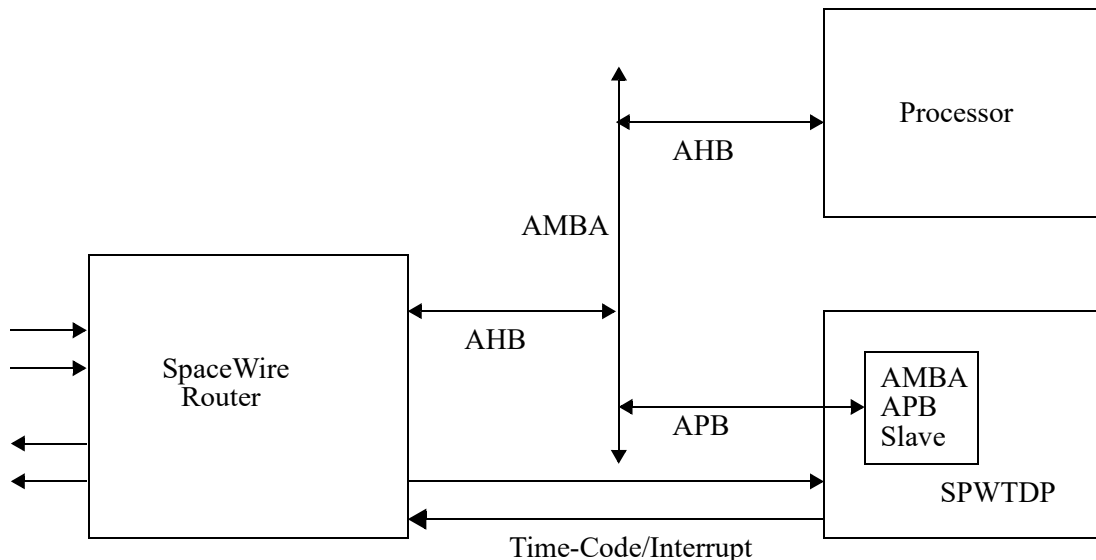
Figure 44. Block diagram
