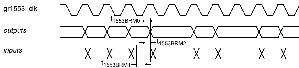
Figure 69. Timing waveforms
