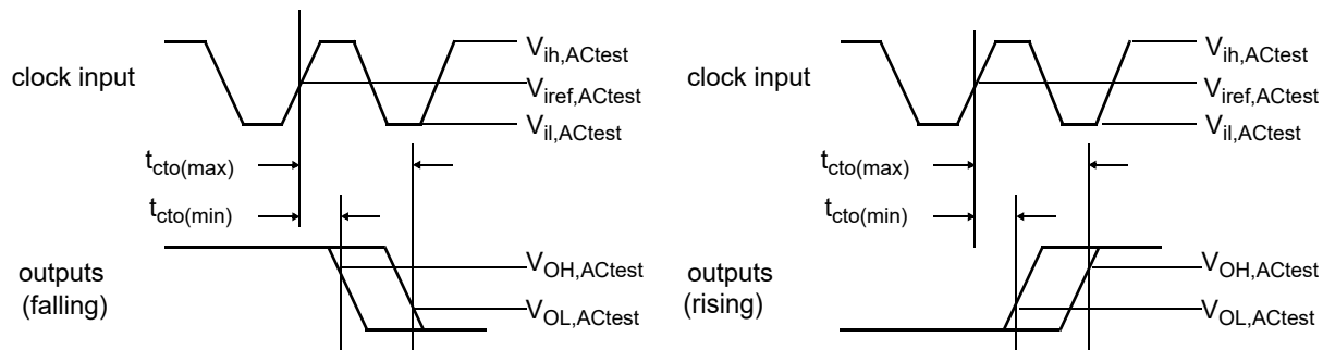
Figure 57. Clock-to-out definition
