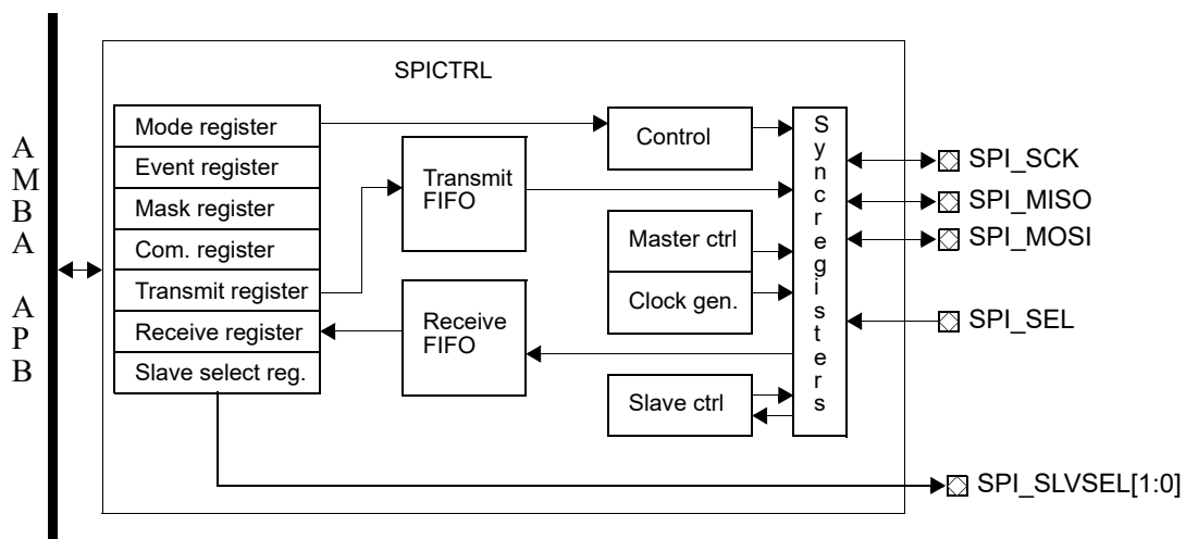
Figure 42. Block diagram
