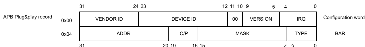
Figure 55. APB plug&play information
