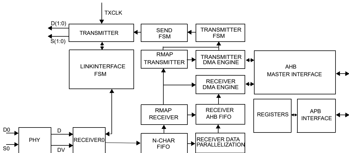
Figure 47. Block diagram
