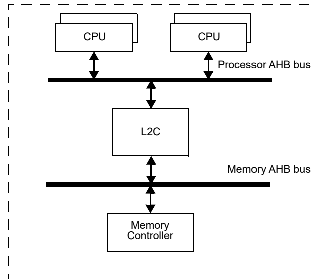
Figure 9. Block diagram
