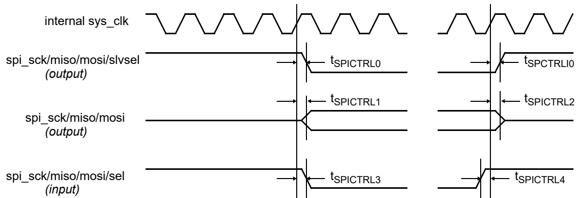
Figure 75. Timing waveforms
