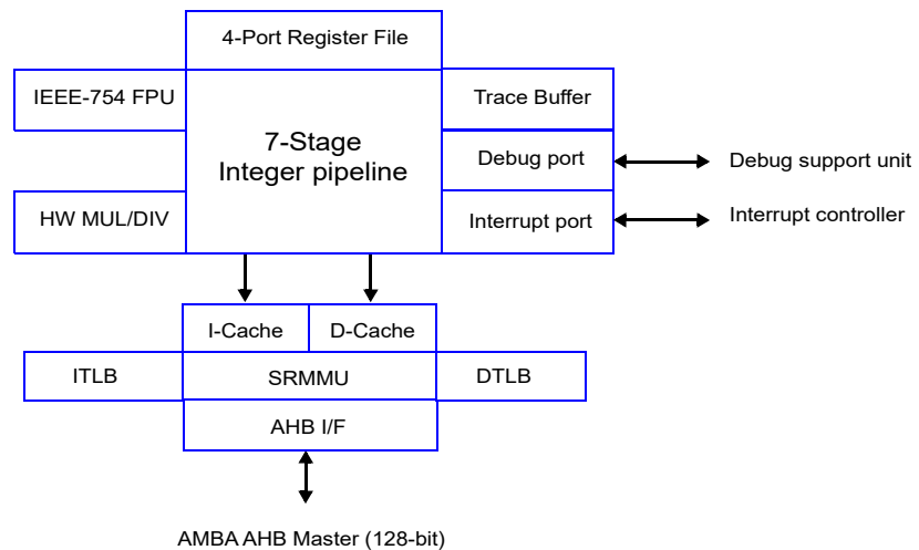
Figure 3. LEON4 processor core block diagram
