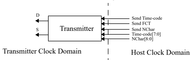
Figure 49. Schematic of the link interface transmitter.
