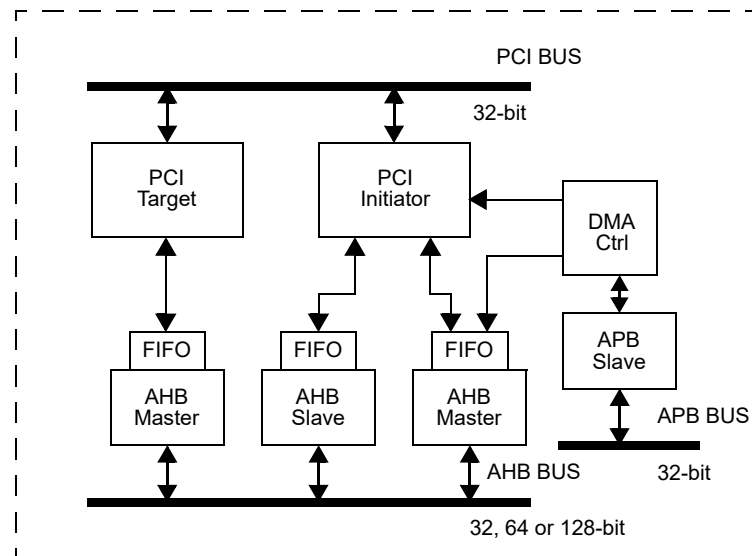
Figure 18. Block diagram
