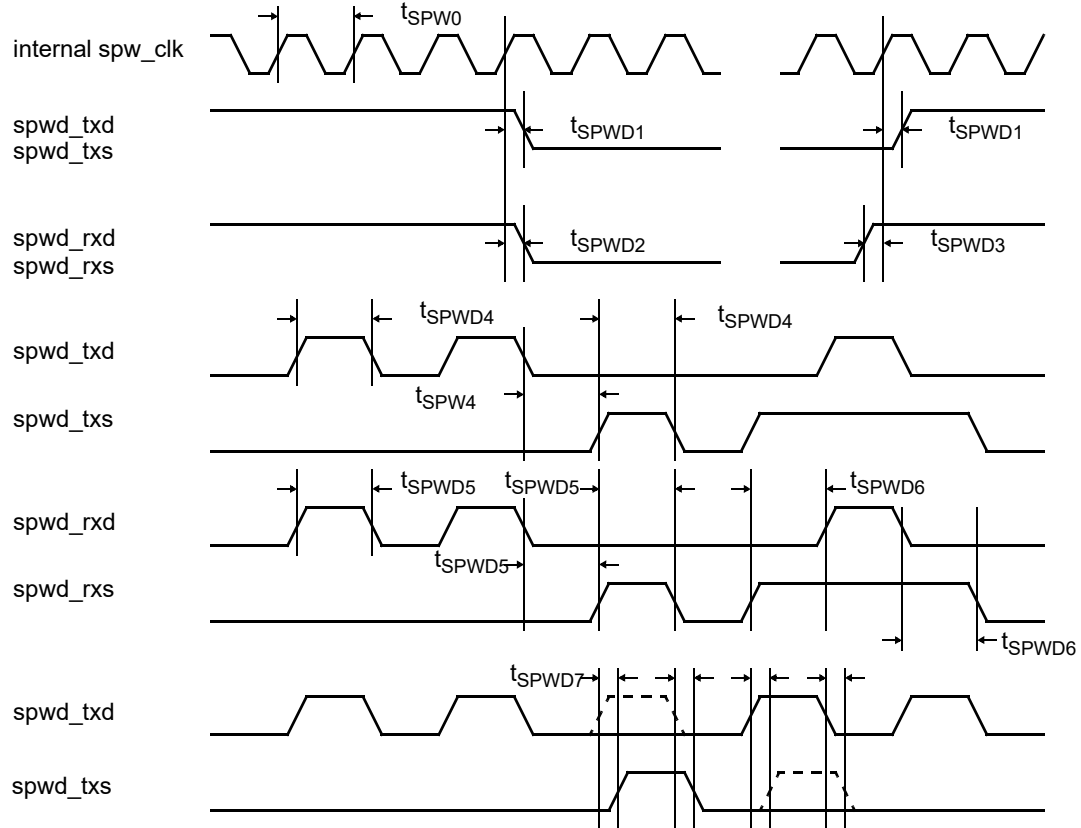
Figure 67. Timing waveforms
