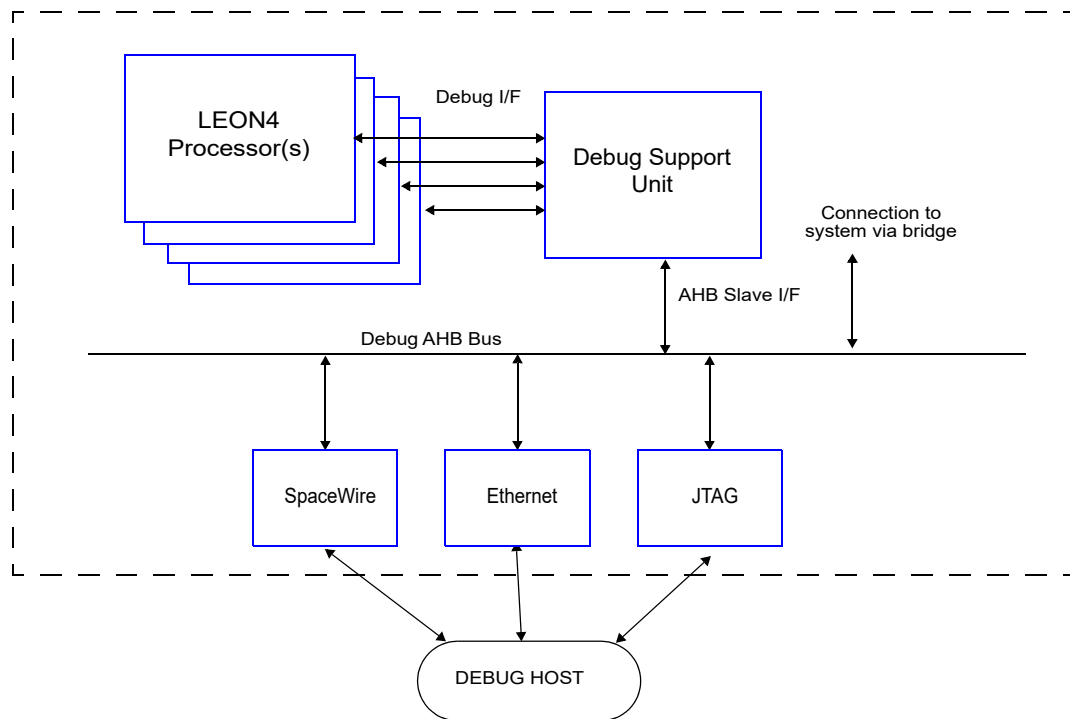
Figure 45. LEON4/DSU Connection
