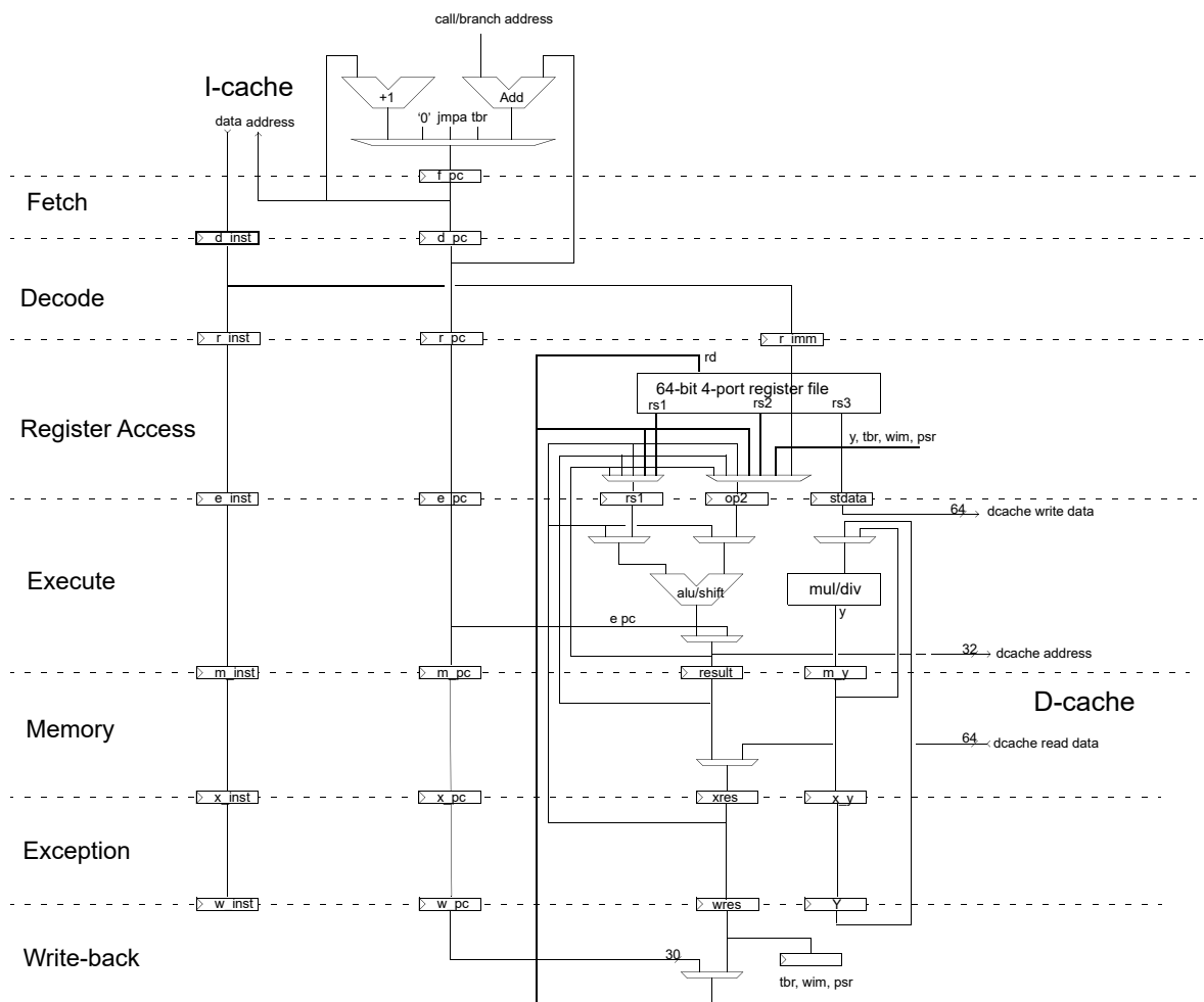
Figure 4. LEON4 integer unit datapath diagram
