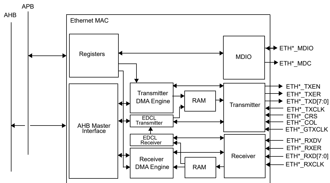
Figure 17. Block diagram of the internal structure of the GRETH GBIT
