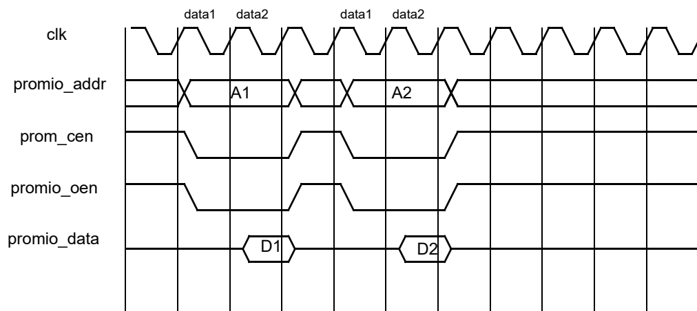
Figure 24. Prom non-consecutive read cycles.
