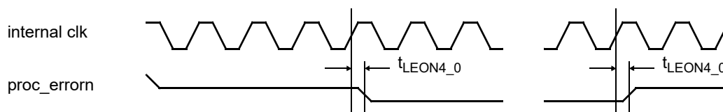
Figure 60. Timing waveforms
