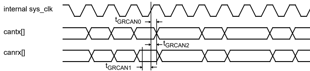
Figure 76. Timing waveforms
