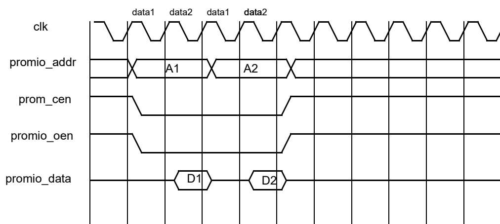
Figure 25. Prom consecutive read cycles.
