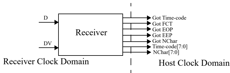
Figure 50. Schematic of the link interface receiver.
