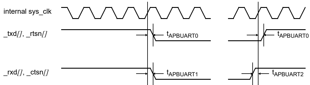
Figure 74. Timing waveforms
