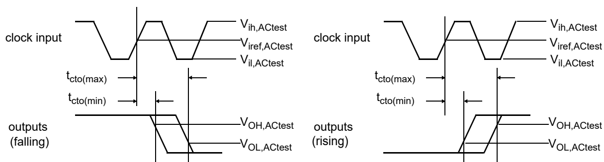
Figure 57. Clock-to-out definition
