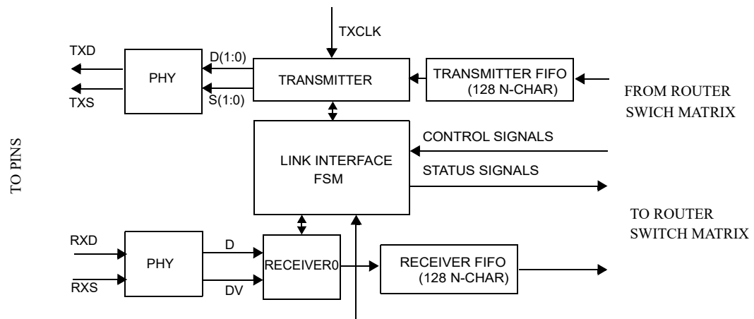
Figure 13. Block diagram
