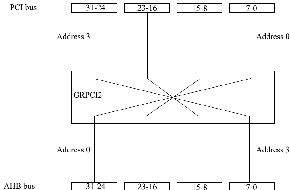
Figure 19. GRPCI2 byte twisting
